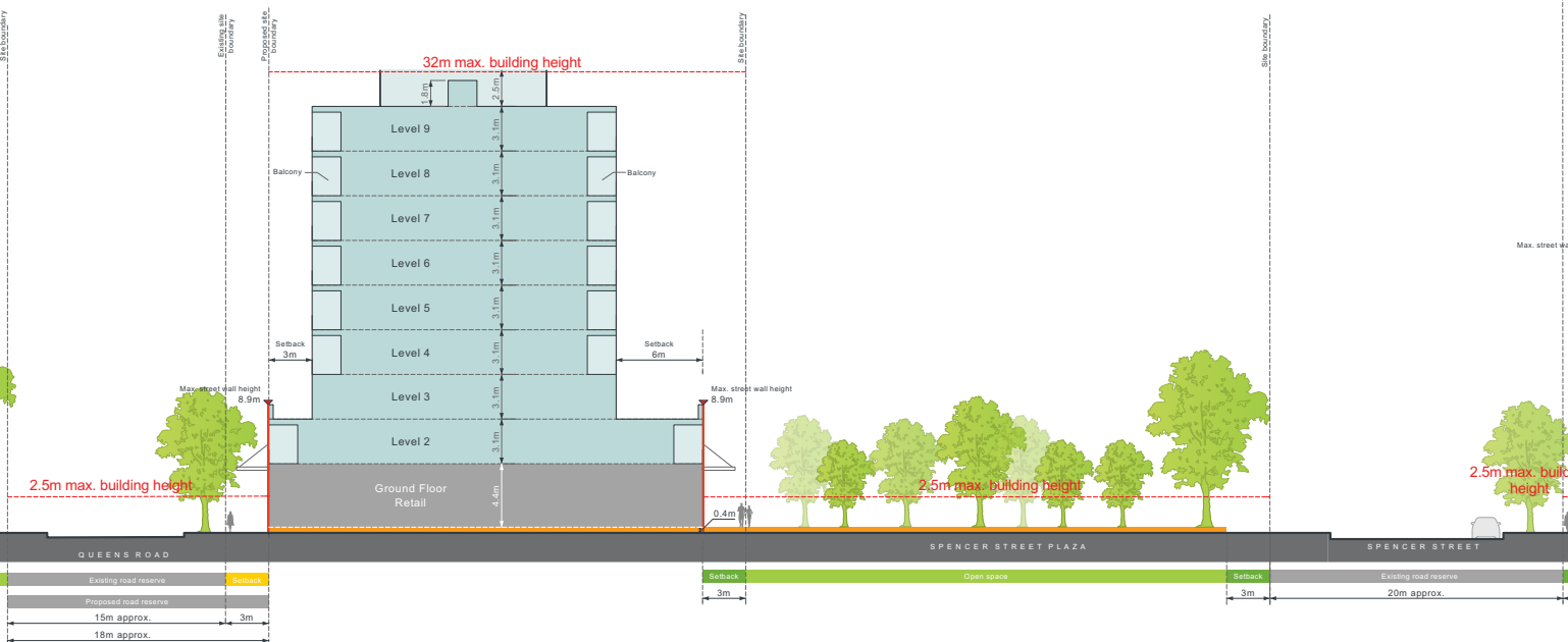
Figure K20-19 Built Form Envelope - Section B
