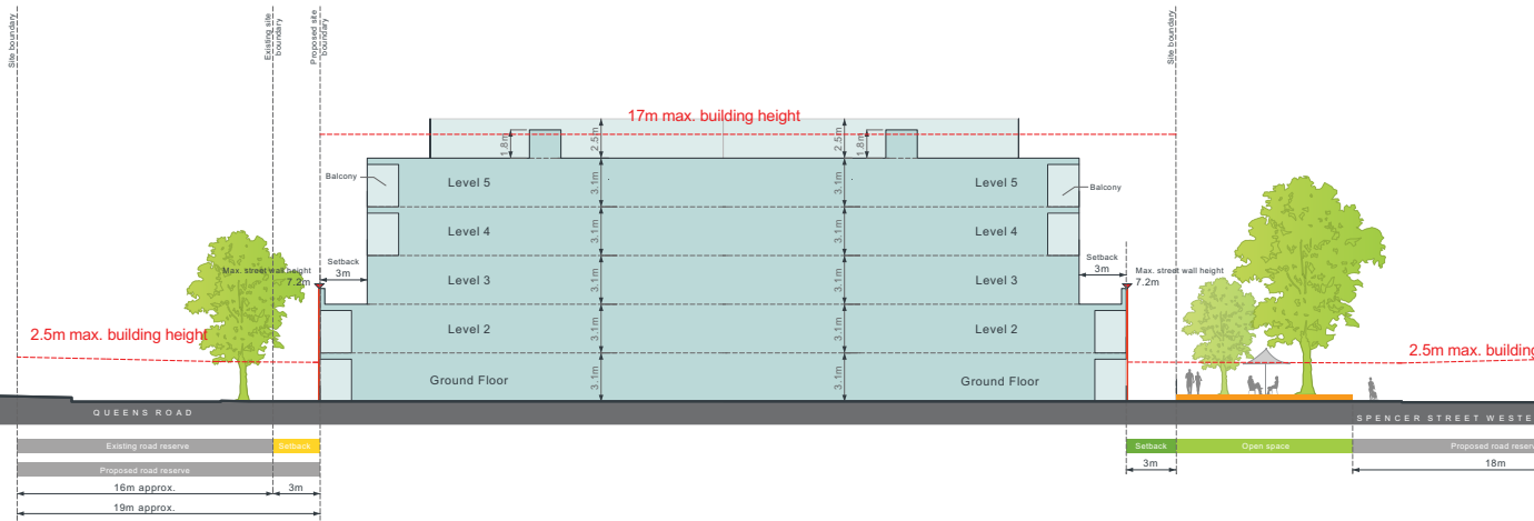
Figure K20-18 Built Form Envelope - Section A
